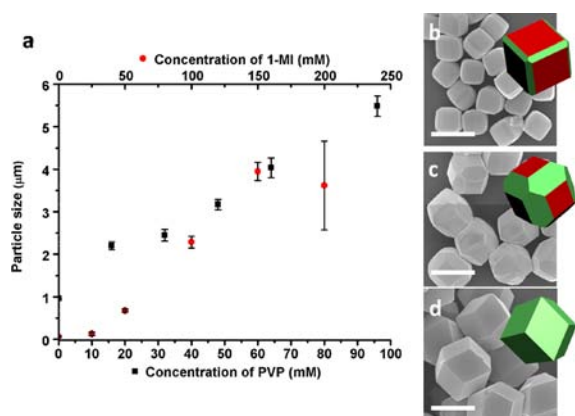
Figure 2. Crystal size and morphology controlled by two capping ligands. (a) Crystal size of ZIF-8 synthesized in the presence of various concentrations of capping ligands, 1-MI and PVP. Black dots show dependence of particle size on PVP concentration (1-MI is fixed at 100 mM), while red dots show dependence on 1-MI concentration (PVP is fixed at 32 mM). Concentrations of \text{Zn}(\text{NO}_3)_2 \cdot 6\text{H}_2\text{O} and Hmim were fixed at 25 and 100 mM, respectively. SEM images of ZIF-8 crystals crystallized for (b) 1, (c) 3, and (d) 20 h ( 3.7\ \mu\text{m} in size). Scale bars = 3\ \mu\text{m} . Schematic representations of the three crystal morphologies are shown as insets.
