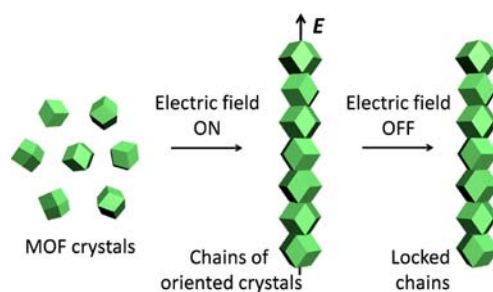
Figure 1. Scheme according to which electric field assembles MOF crystals into chains with orientational order, the particles remaining locked into stable chains when electric field is switched off.
